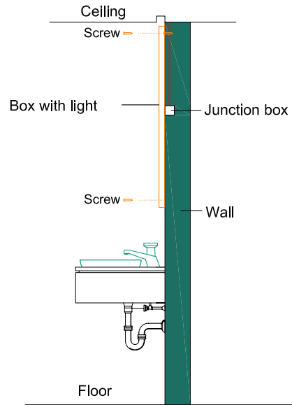
2 To fix the light box to the determined location of wall by screws
